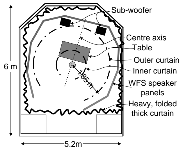
Figure 1: Plan view of the experimental set-up.
